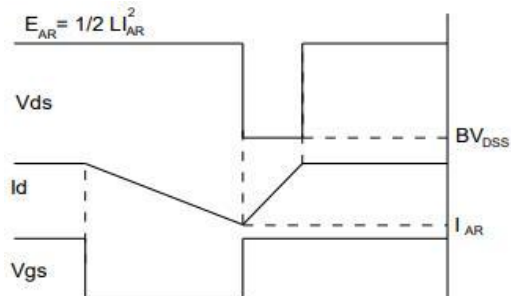
Fig.3-2 Avalanche waveform
