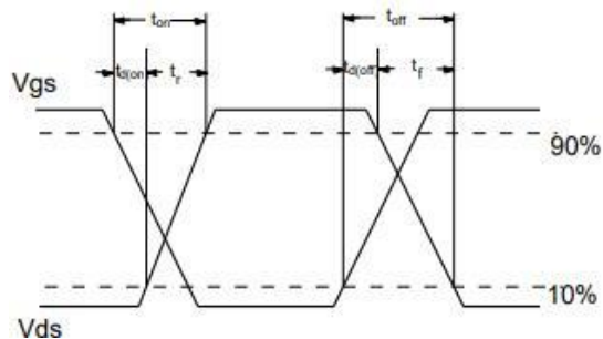
Fig.1-2 Switching Waveform
