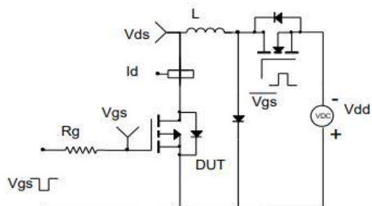
Fig.3-1 Avalanche test circuit
